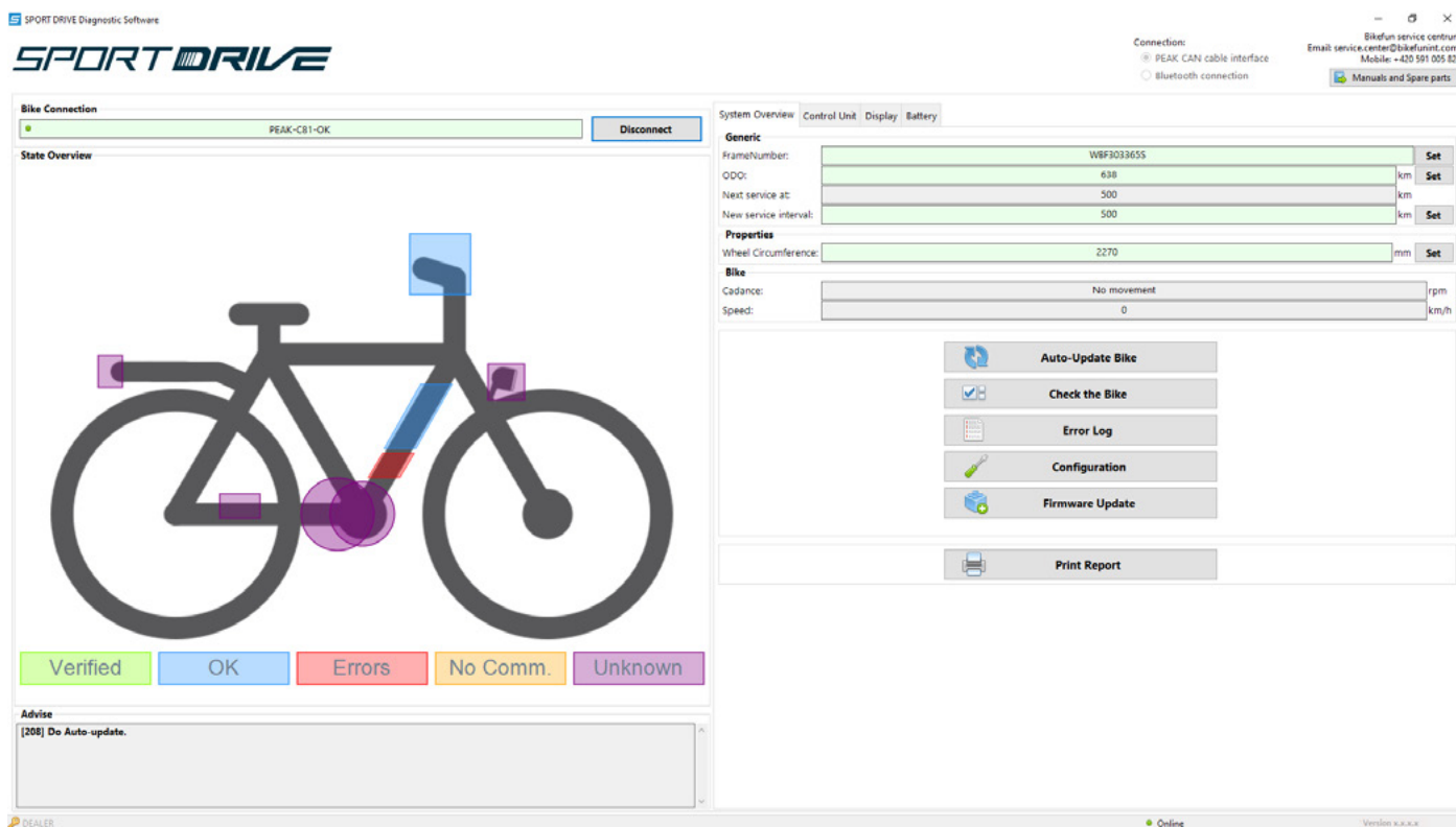
Figure 3.20 Auto-update – Tips
