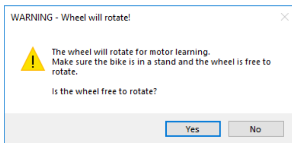
Figure 3.21 Auto-update – Warning
