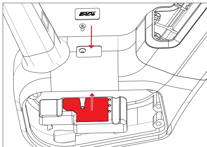
Figure 4.36 Control unit assembly
