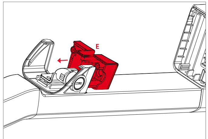
Figure 4.23 Inserting the middle part
