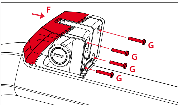
Figure 4.24 Mounting the front part
