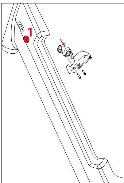
Figure 4.33 Lock iassembly1
