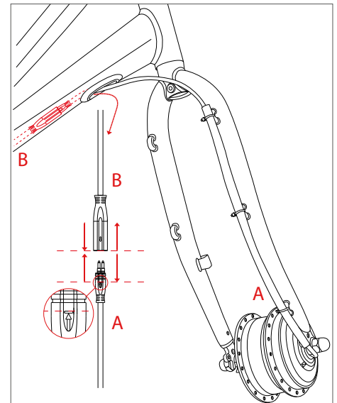
Figure 4.1 Motor cable connection and disconnection – front motor
