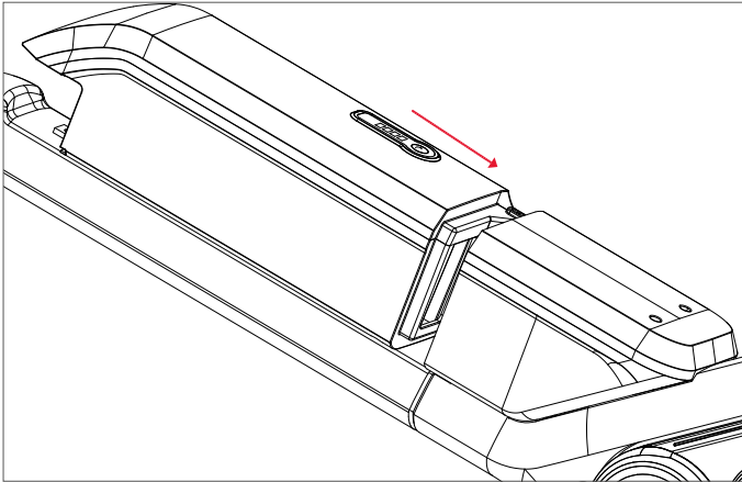
Figure 4.20 Lock assembly – battery insertion
