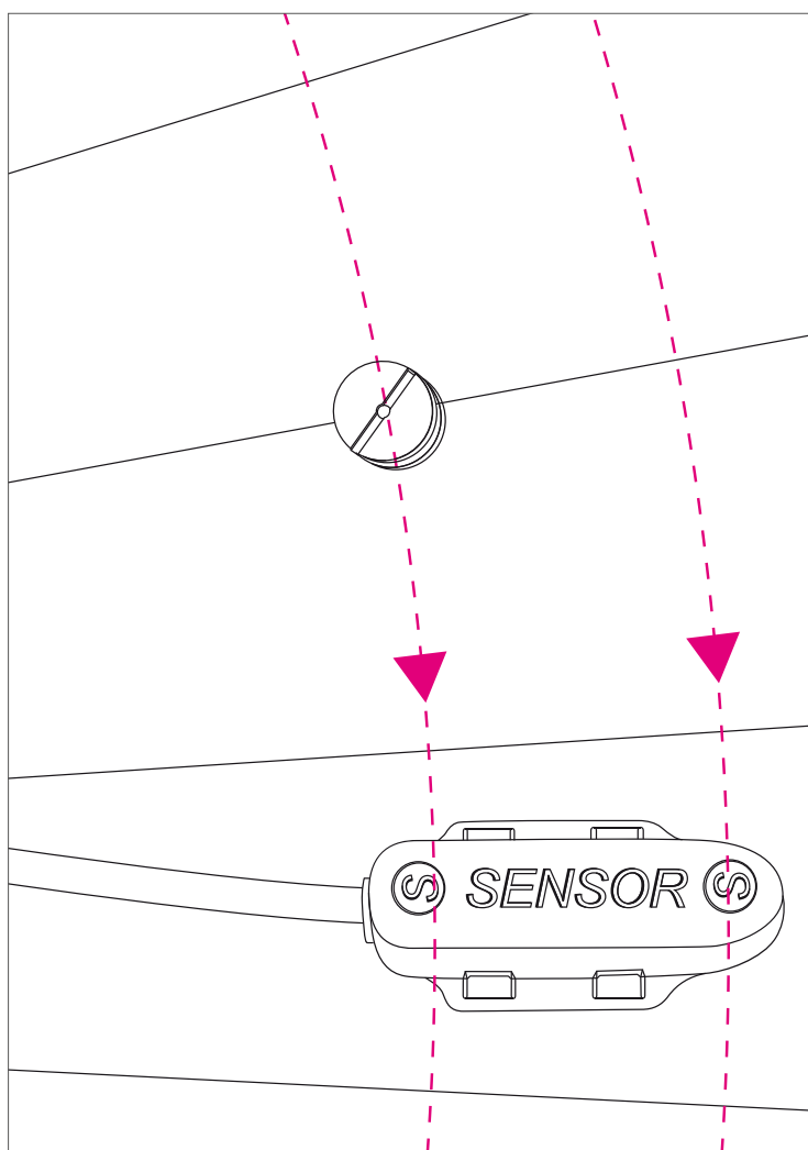
Figure 4.43 Magnet position relative to the sensor
